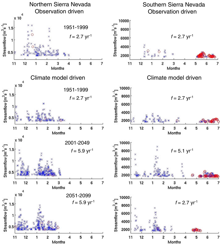
Fig. 5 Floods in Californian Northern Sierra Nevada ( Left ) and Southern Sierra Nevada ( Right ). Panels on first row shows floods using observed meteorology driven VIC simulated streamflows from the period 1951–1999. Second and third row panels show floods using downscaled CNRM CM3 driven VIC simulated streamflows from periods 1951–1999, 2001–2049 and 2051–2099. Numbers ( f ) in each panel indicate frequency of the floods per year on average. In the figure, “X” symbols are precipitation-driven floods and red circles are snowmelt driven floods. Flood is defined if streamflow in a given day for the period November through July is larger than 99 percentile value computed from the time period 1951–1999
