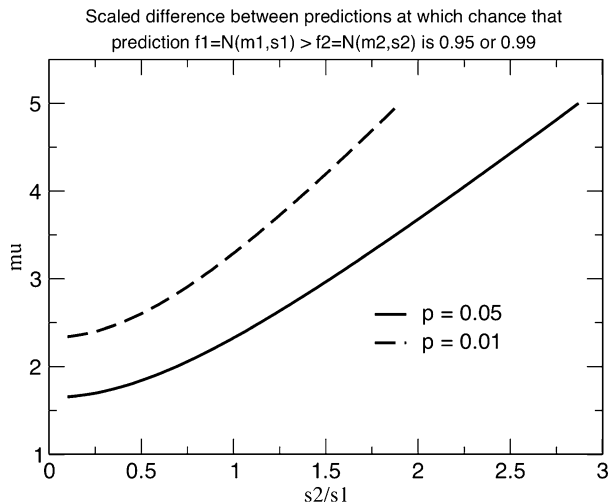
Fig. 8 Values \mu = (m_2 - m_1) / s_1 as a function of s_2 / s_1 where the probability that f_1 \sim N(m_1, s_1) is greater than f_2 \sim N(m_2, s_2) is 0.95 or 0.99
