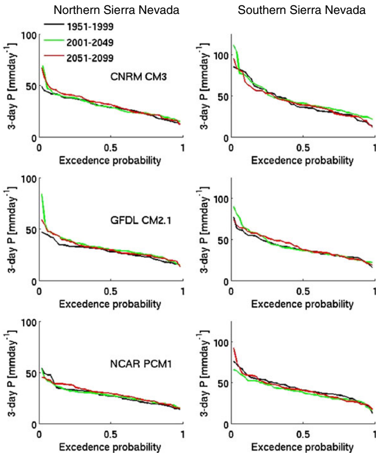
Fig. 2 Probability distributions for 3-day annual maximum precipitation from CNRM CM3, GFDL CM2.1 and NCAR PCM1 GCMs. Climate change period (2000–2099) from SRES A2 scenarios. 1951–1999 period is from GCM simulated historical period. ( Left ) Northern Sierra Nevada, ( Right ) Southern Sierra Nevada
