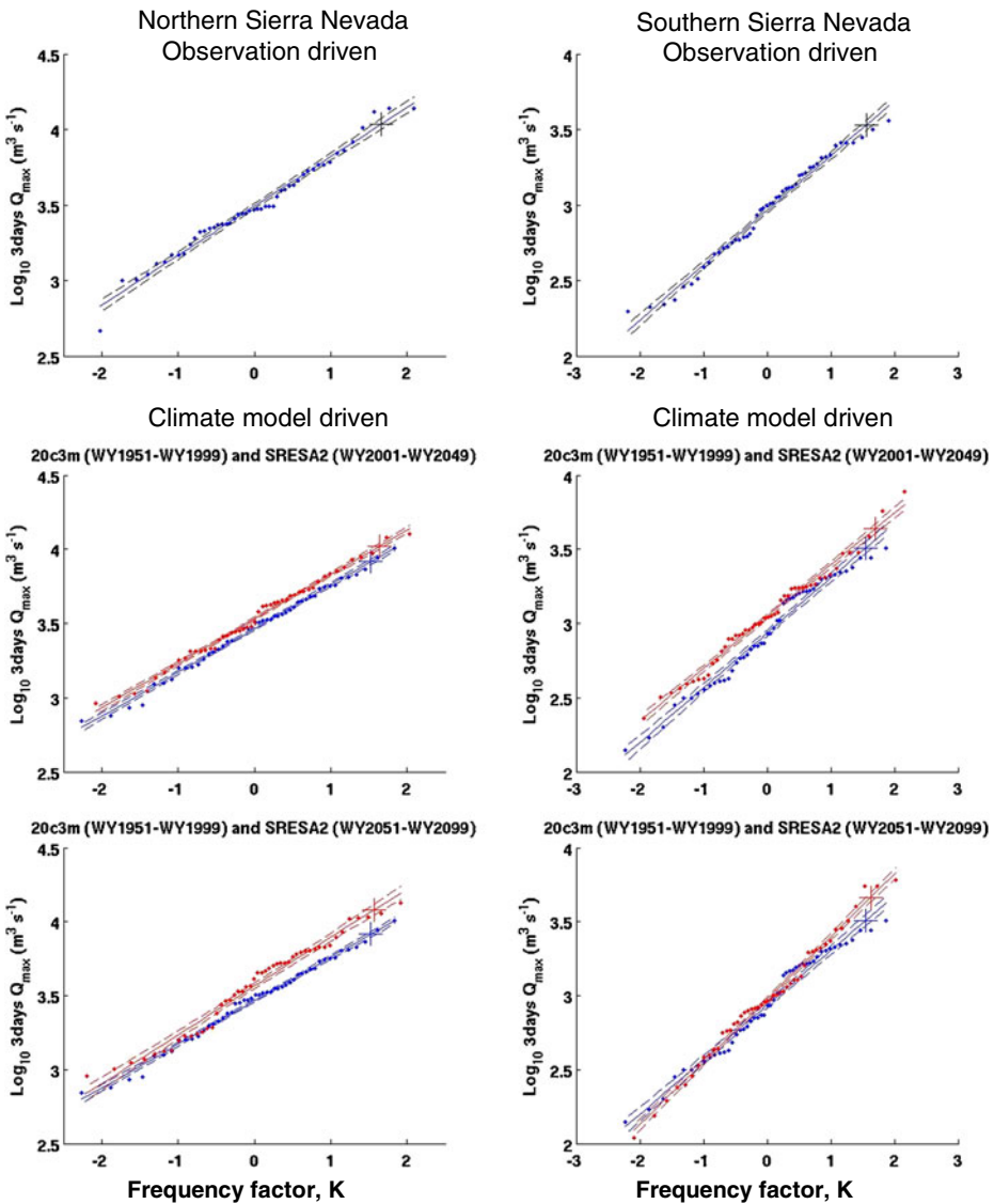
Fig. 4 Frequency of the three-day annual maximum streamflows. Log Pearson III distributions have been fitted to each flood series. Dotted curves: confidence limit for regression line (at 0.01 confidence level). Panels on first row shows flood frequency curves developed using observed meteorology driven VIC simulated streamflows from the period 1951–1999. Second and third row panels compares flood Frequency curves developed using downscaled CNRM CM3 driven VIC simulated streamflows from period 1951–1999 (blue curves) with time periods 2001–2049 and 2051–2099. In the figures, “+” symbol mark flood magnitude with 20-years return period. (Left) Northern Sierra Nevada, (Right) Southern Sierra Nevada
