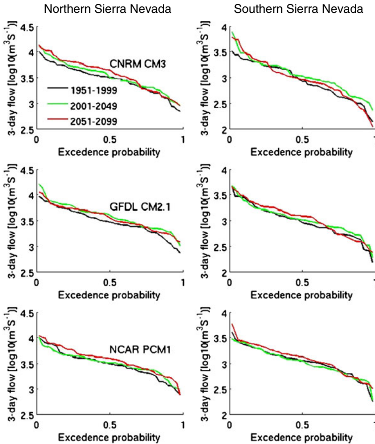
Fig. 3 Same as Fig. 2, except using 3-days maximum annual streamflows as simulated by downscaled meteorology from CNRM CM3, GFDL CM2.1 and NCAR PCM1 GCMs
