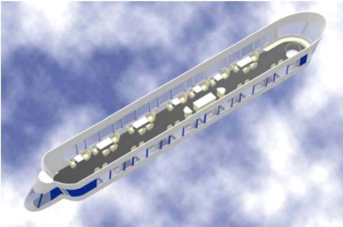
The ZET gondola features 14 comfortable seating groups and a panoramic bar at the aft end (right) of the gondola. The passengers enter and exit via stairs under the cockpit (left). Source: ZET
