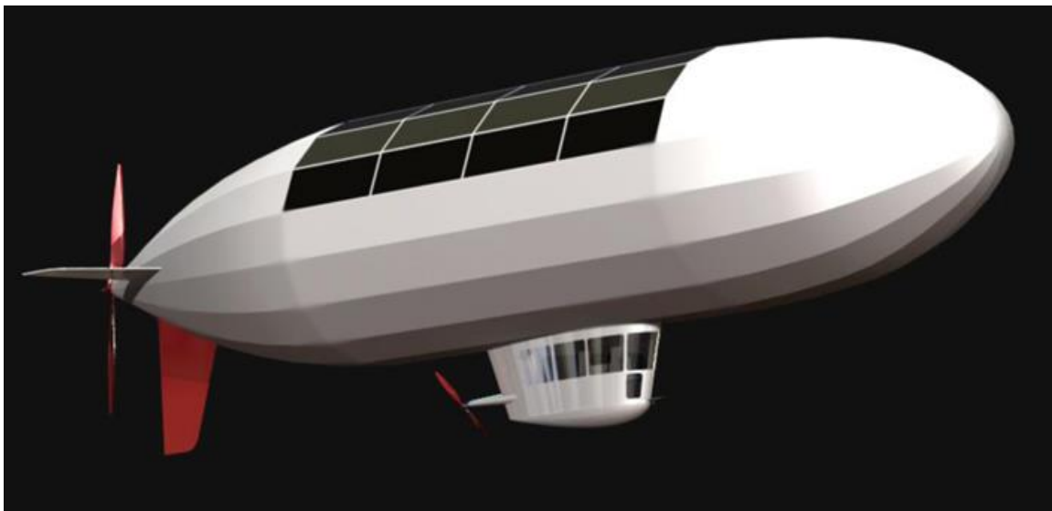
General arrangement of the Sunship airship. Source: https://www.technologicvehicles.com/fr/
