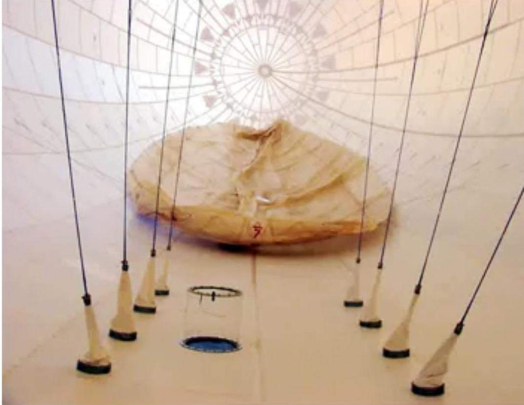
Inside the Sky Dragon envelope, looking forward from above the gondola. Note the catenary cables carrying the weight of the gondola into the upper surface of the envelope. Above: deflated forward ballonet. Below: partially inflated forward ballonet. Source: Aeros
