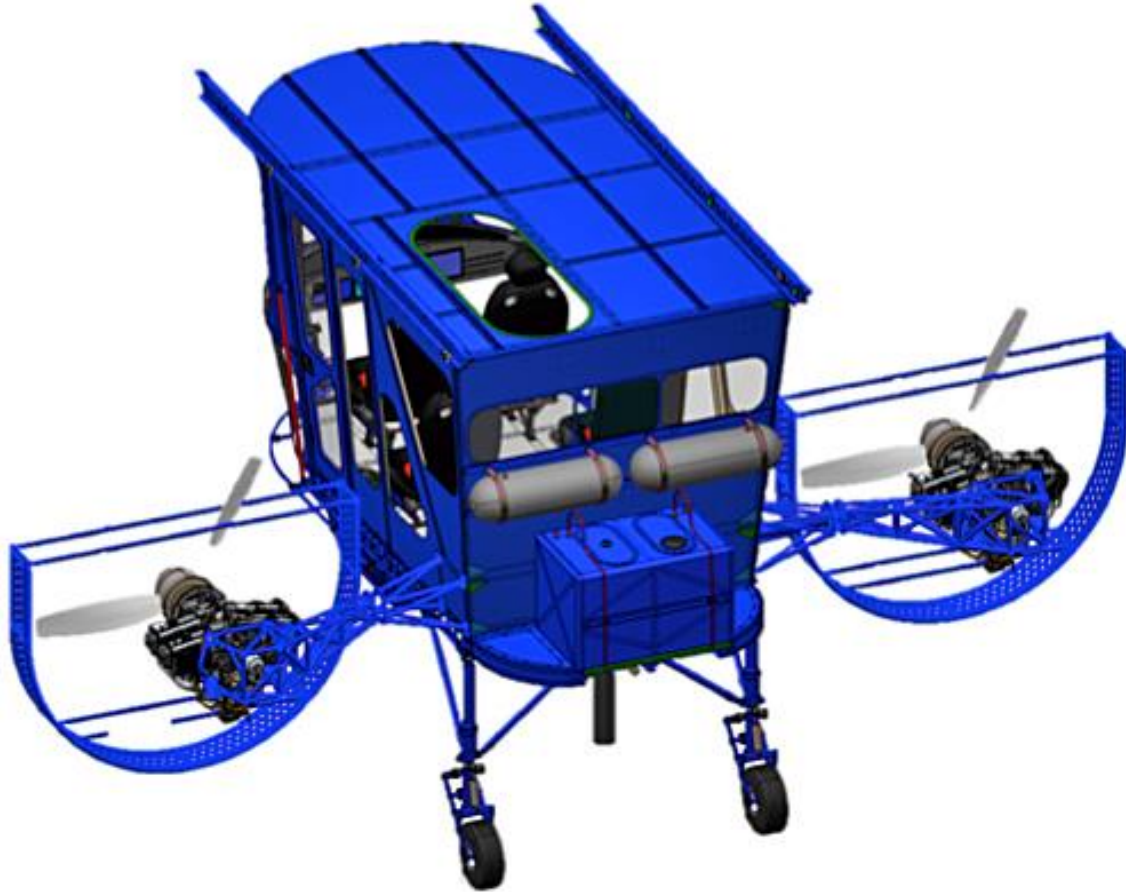
Aeros 40E gondola (viewed from rear quarter) and vectored propeller arrangement. Source: Aeros
